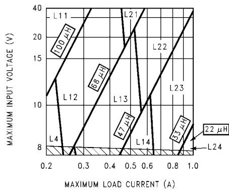
FIGURE 4. LM2672-3.3
